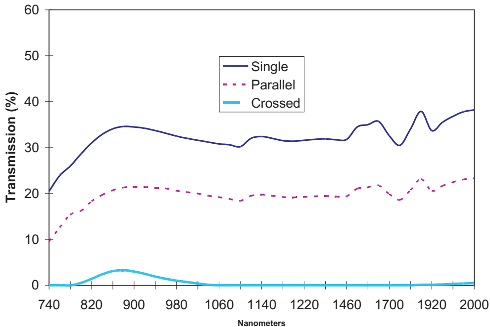
Spectral Transmission 3M HR
