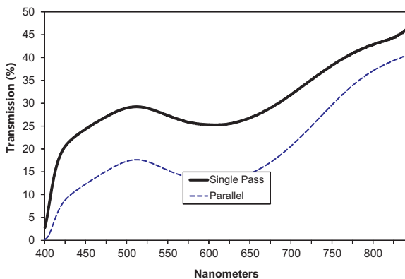
Single and Parallel Transmission in Unpolarized Light
