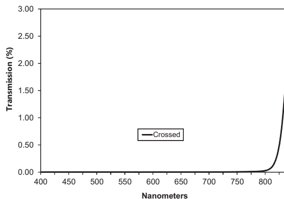
Crossed Transmission in Unpolarized Light
